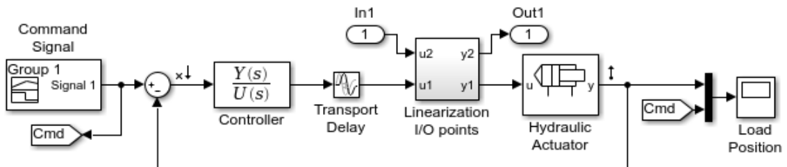
Hydraulic Actuator with Digital Position Controller
